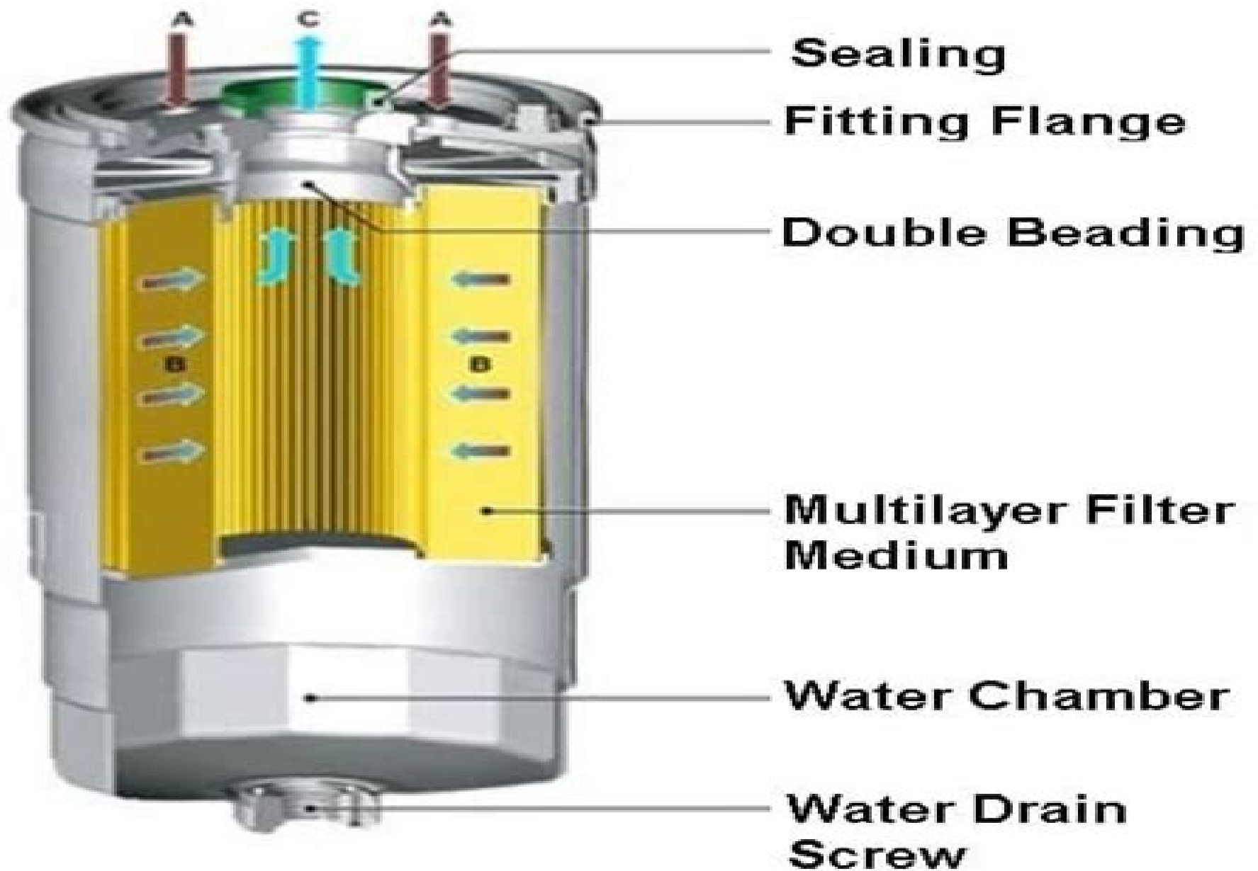
Fuel Filter
